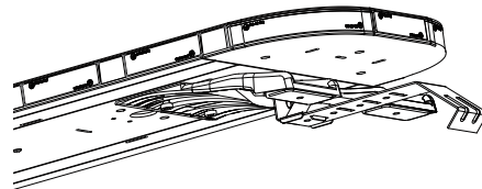
Gutter Mounting By Brackets for sky 42, sky 48, sky 54
