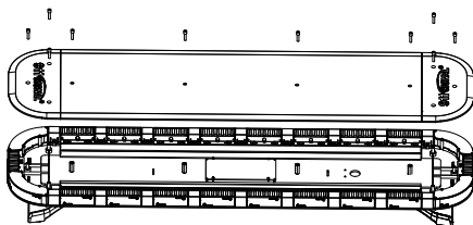
1、 Secure extender with screws the top cover
